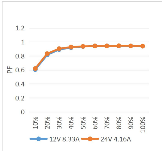
Power factor characteristic curve
