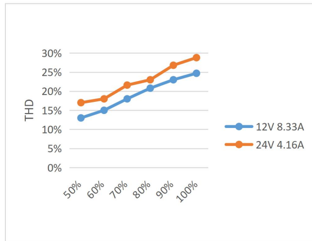
Total harmonic distortion characteristic curve
