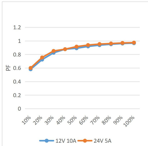
Power factor characteristic curve
