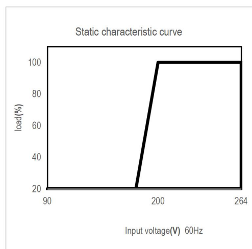
Static characteristic curve
