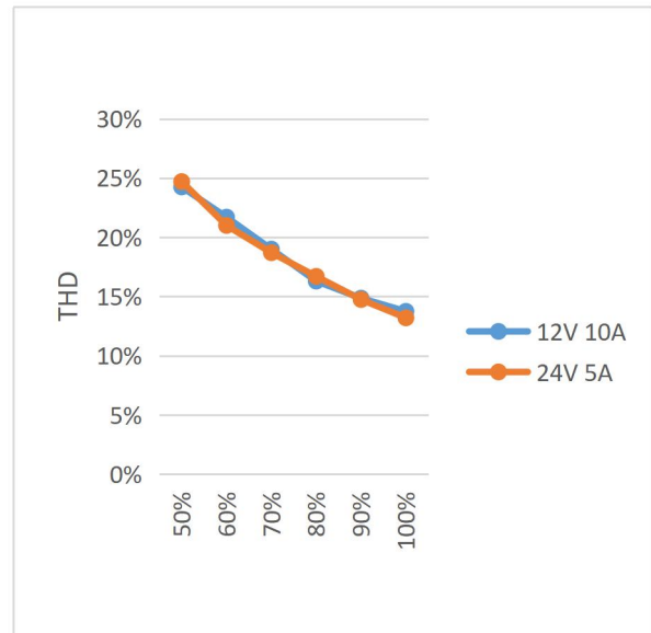
Total harmonic distortion characteristic curve
