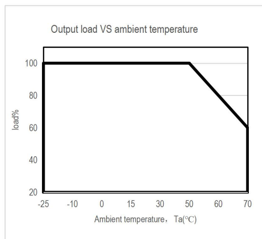
Output load VS ambient temperature
